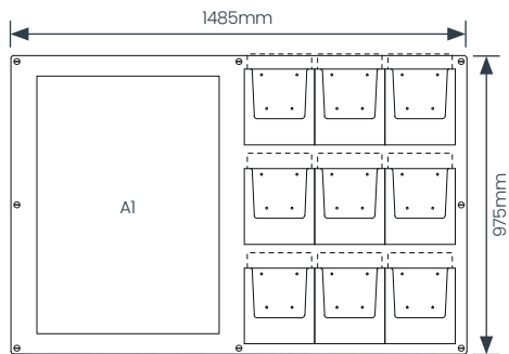
Acrylic Back Panel
