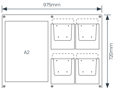
Acrylic Back Panel
