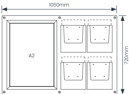
ACM Back Panel
